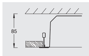
Installation simultaneously with the false ceiling, minimum void of 85 mm from the structure's lower edge.
