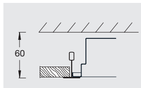
Installation simultaneously with the false ceiling, minimum void of 60 mm from the structure's lower edge.
