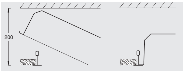
Installation following false ceiling mounting, supported by the exposed structure, minimum void of 200 mm from the structure's lower edge.
