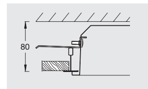
Minimum void of 80 mm from the structure's lower edge. Luminaires on request, installed flush with bracket accessory 15 ZH.
