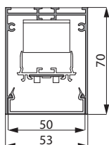
with cover 070, 072 and 090
