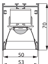
with louver 990 and 991
