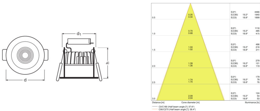
SPOT DK FIX 7 W 3000 K IP44 WT
