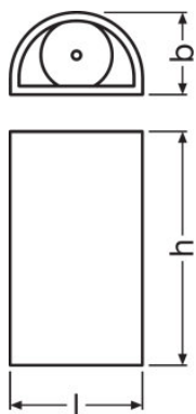
O FACADE UPDOWN 12 W 3000 K IP54 GY, O FACADE UPDOWN 12 W 3000 K IP54 WT
